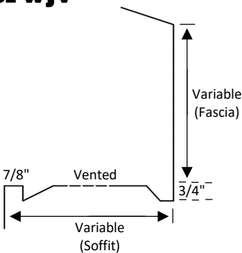
Drop-Face Eave Soffit/Fascia with J Vented
