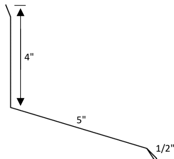
End Wall
