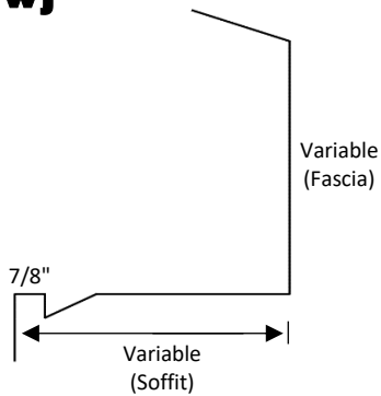
Eave Soffit/Fascia with J
