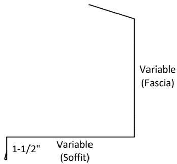
Eave Soffit/Fascia NO J
