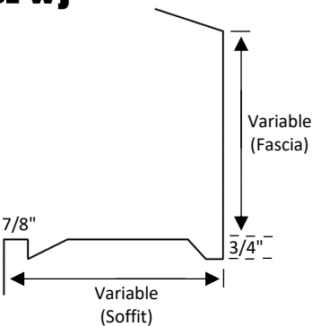
Drop-Face Eave Soffit/Fascia with J
