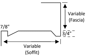
Drop-Face Gable Soffit/Fascia with J
