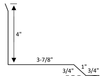
Side Wall
