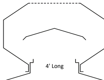
4ft Ridge Vent (High Flow)
