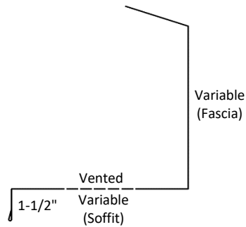
Eave Soffit/Fascia NO J Vented
