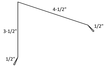
Ridge Drip
