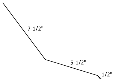
Pitch Change
