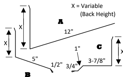
Chimney Kit (Custom Height)
