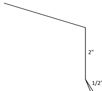
Eave Drip 2"
