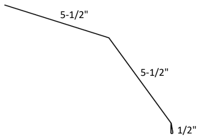
Gambrel Flashing
