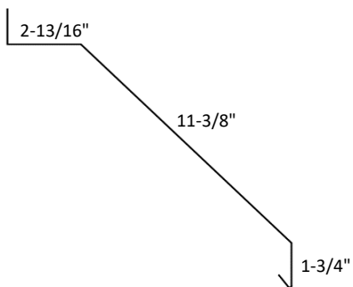
Double Track Cover
