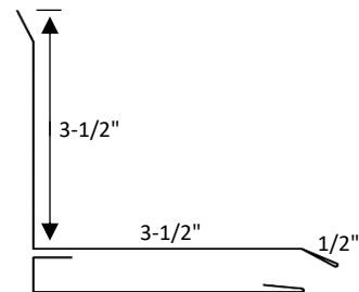
Metal Line Side Wall with Gal. Inside J
