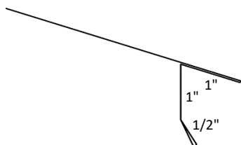
Extended Eave 1"
