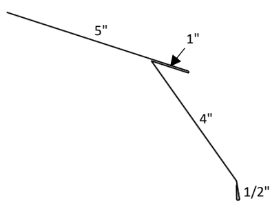
Metal Line Gambrel Flashing
